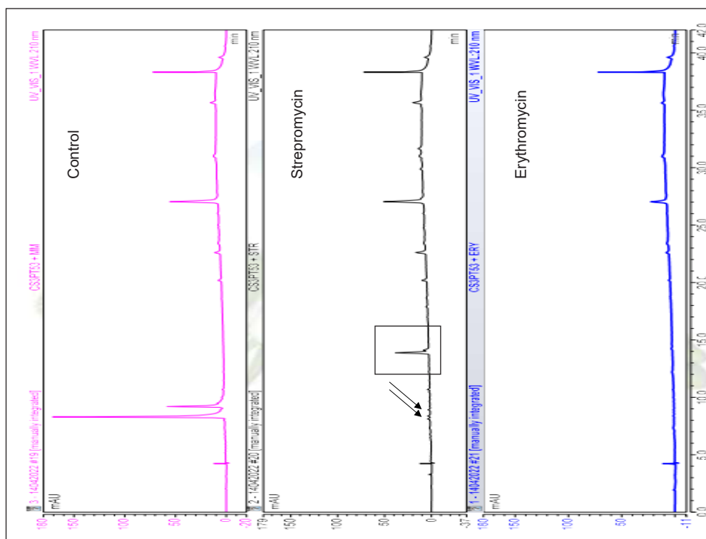
Figure 4. HPLC profiles of isolate CS3PT53 extracts at 210 nm
